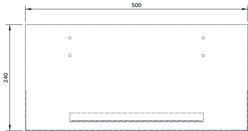
TOP VIEW Scale 1:5; looking down (along -Z)
