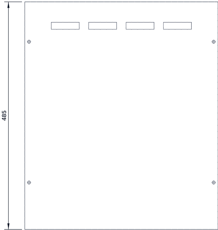
FRONT VIEW Scale 1:5; looking at the front (along +Y)
