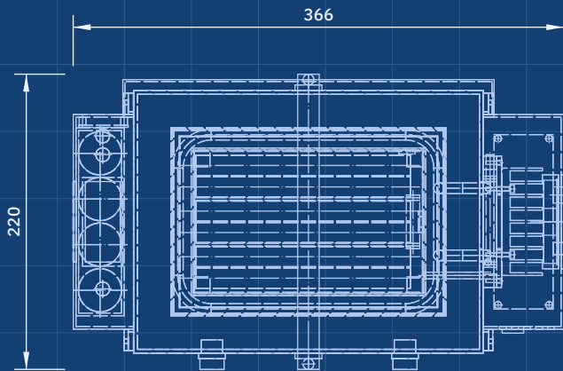
TOP VIEW Scale 1:5; looking down (along -Z)
