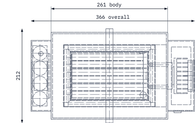
TOP VIEW Scale 1:5; looking down (along -Z)
