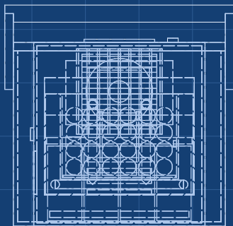
RIGHT VIEW Scale 1:5
