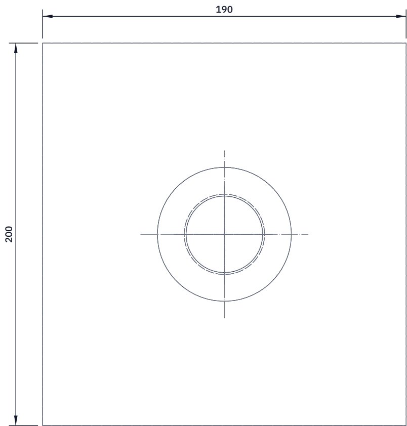
TOP VIEW
