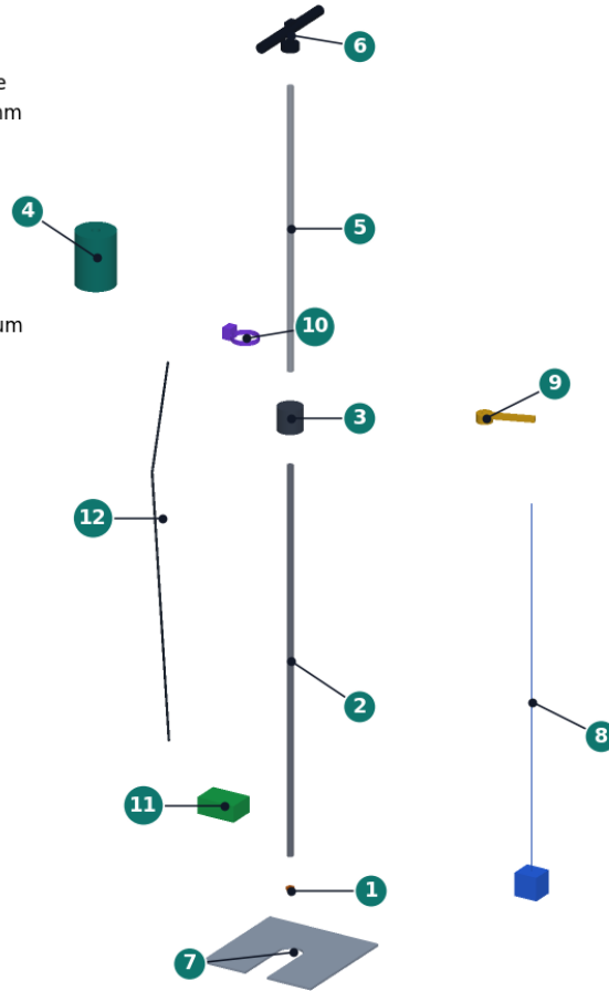
Figure 3. Exploded view with numbered callouts matching the BOM. The carry bag, hardware and the optional extraction lever and extension rod are not shown.
