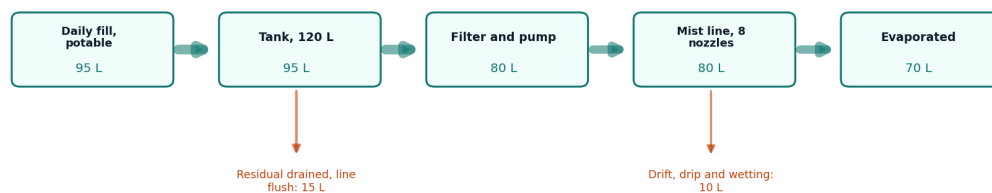
Figure 2. Daily water flow on the design day, in liters. All values are estimates.
