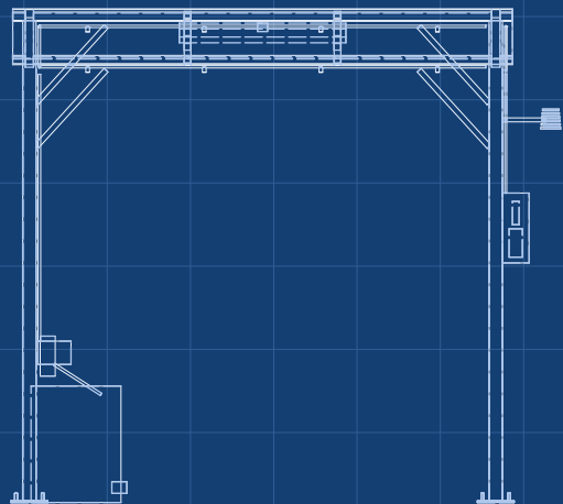
FRONT VIEW Scale 1:50
