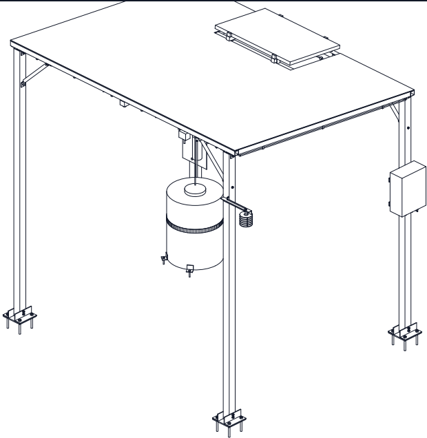
ISOMETRIC VIEW
