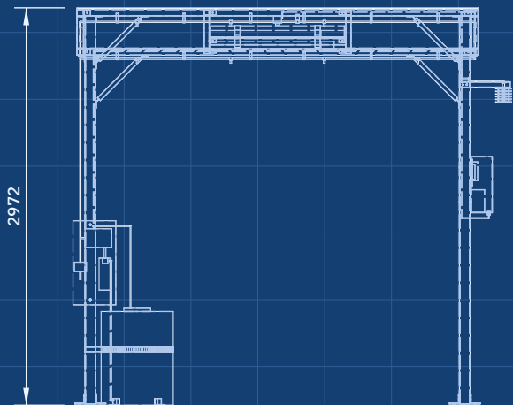
FRONT VIEW Scale 1:50; looking at the front (along +Y)
