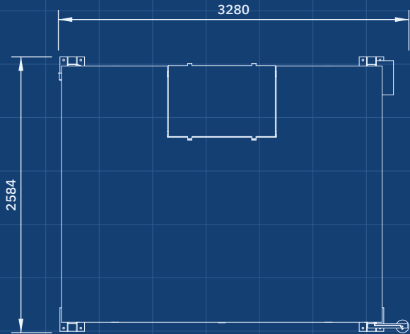
TOP VIEW Scale 1:50; looking down (along -Z)
