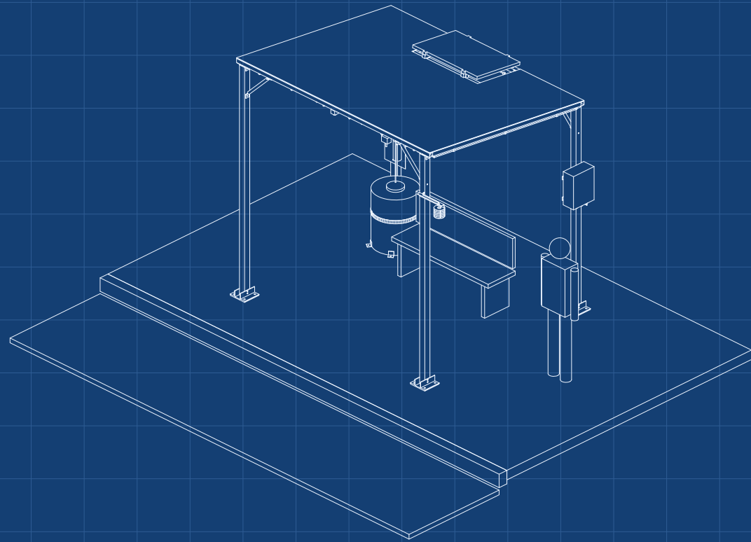
ISOMETRIC VIEW Not to scale; figure is a 1.75 m person; seen from the front right and above, about 30 deg elevation
