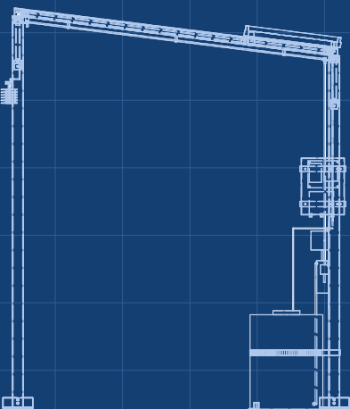
RIGHT VIEW Scale 1:50; looking at the right side (along -X)
