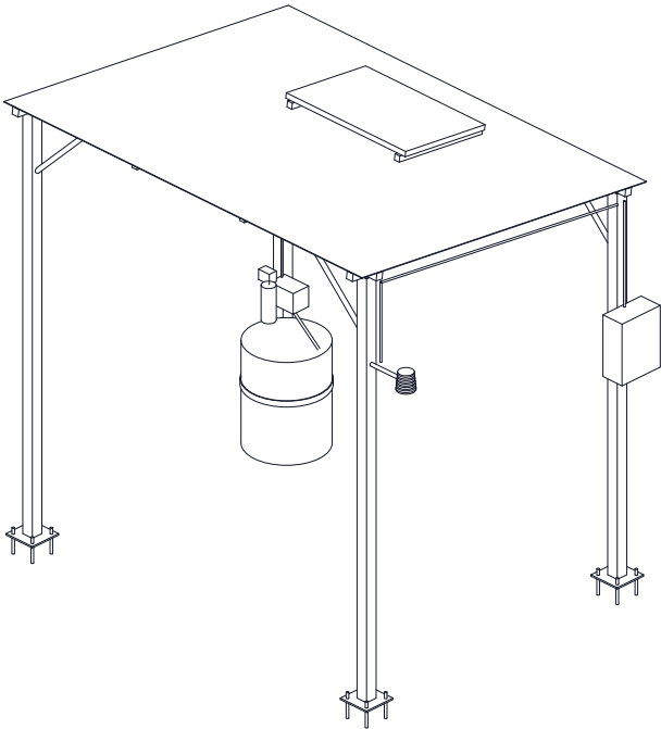
ISOMETRIC VIEW
