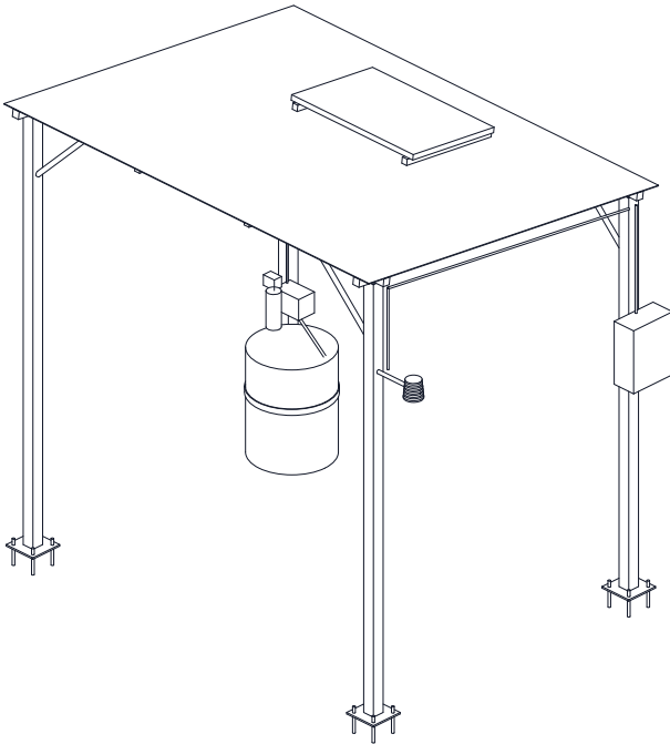
ISOMETRIC VIEW
