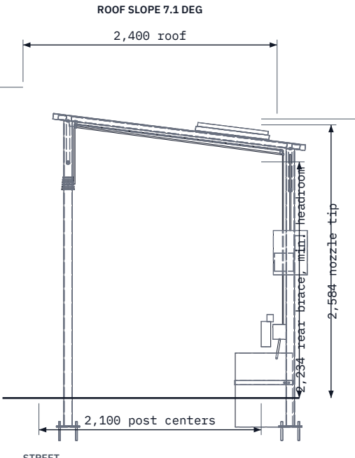
RIGHT VIEW
