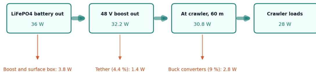
Figure 2. Power flow while driving and profiling, in watts, from CVC-CAL-001. All values are estimates.
