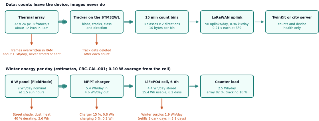
CurbCount: data and energy flow CONCEPT, NOT FOR FABRICATION. Values are estimates from CBC-CAL-001.
