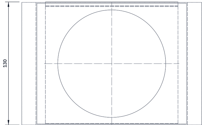
FRONT VIEW Scale 1:2; looking at the front (along +Y)
