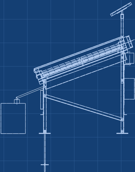
RIGHT VIEW
