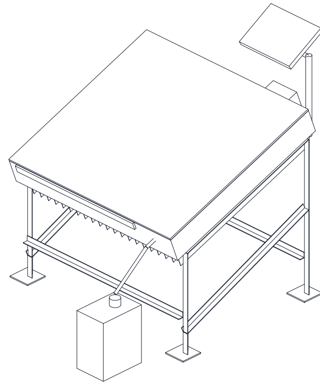
ISOMETRIC VIEW
