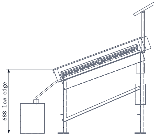
RIGHT VIEW
