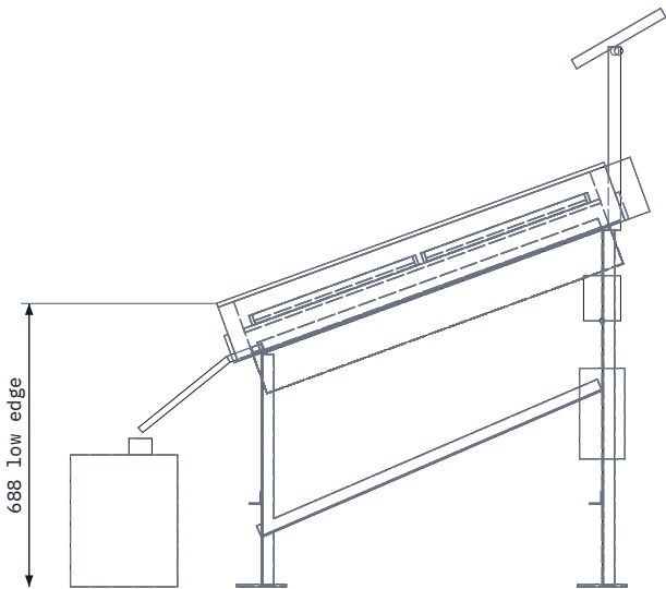
RIGHT VIEW Scale 1:20
