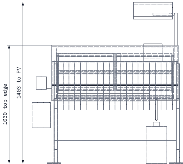
FRONT VIEW Scale 1:20
