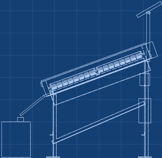
RIGHT VIEW Scale 1:20
