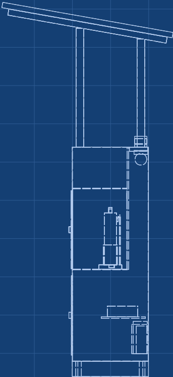
RIGHT VIEW Scale 1:25
