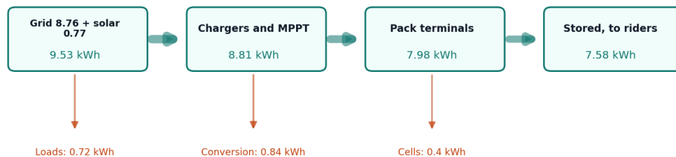
Figure 2. Daily energy at the design duty case of 20 swaps a day with four bays. All values are estimates from DKH-CAL-001.
