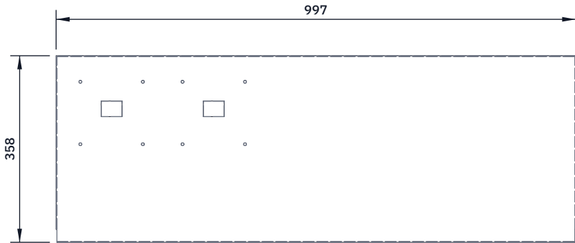
TOP VIEW Scale 1:10; looking down (along -Z)
