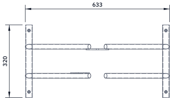
TOP VIEW Scale 1:10; looking down (along -Z)
