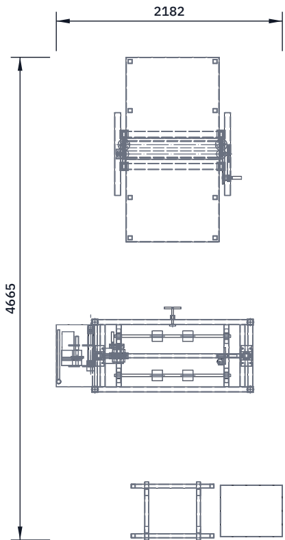
TOP VIEW
