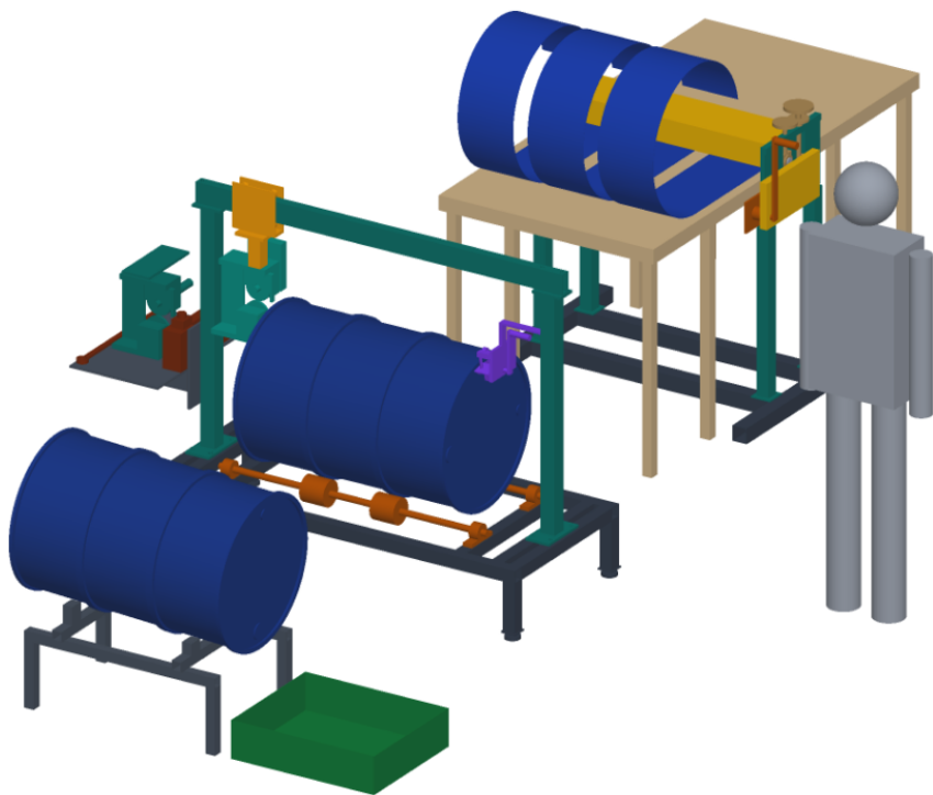
Seen from the front right and above, 24 deg elevation. Front: drain and purge stand; middle: cutting cradle; back: slip roll. Grey figure: 1.75 m person for scale
