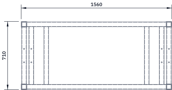
TOP VIEW Scale 1:20; looking down (along -Z)
