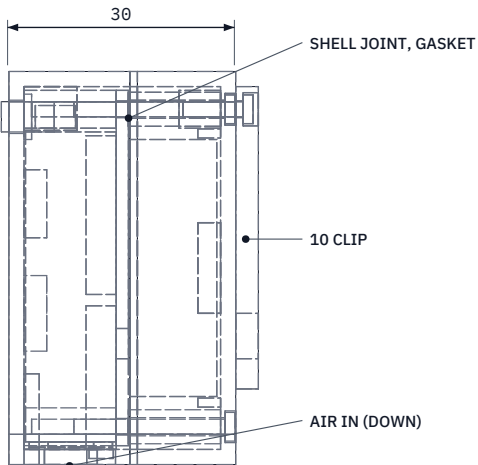
RIGHT VIEW
