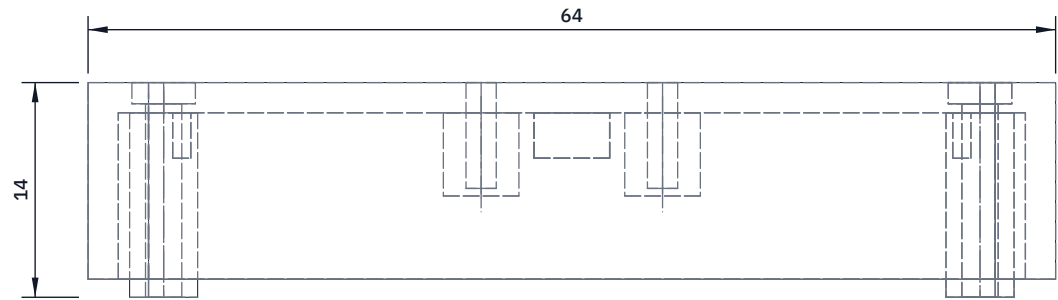
TOP VIEW Scale 2:1; looking down (along -Z)
