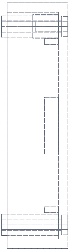
RIGHT VIEW Scale 2:1; looking at the right side (along -X)
