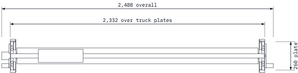
TOP VIEW Scale 1:20
