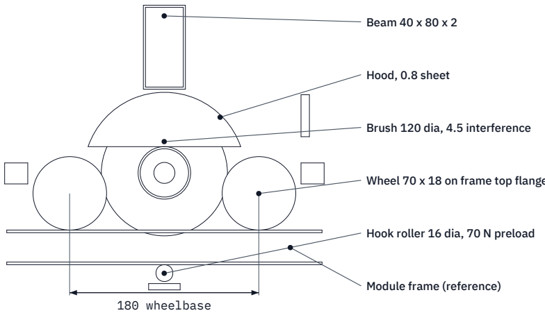
SECTION A-A Scale 1:5; through the upper wheels, looking down the slope
