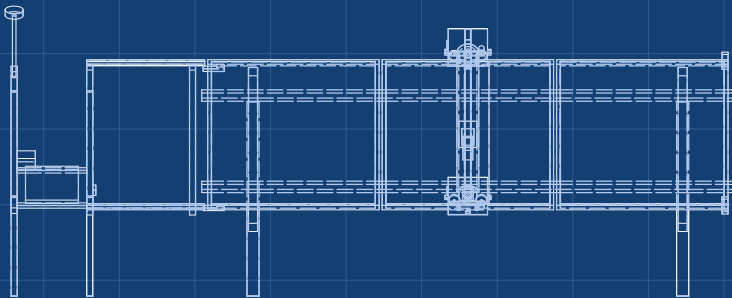
RIGHT VIEW Scale 1:50
