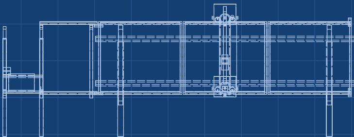
RIGHT VIEW Scale 1:50
