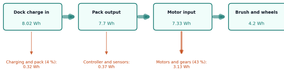
Figure 2. Energy for one out-and-back cycle on the 40 m reference row, in Wh (DRN-CAL-001, F7). All values are estimates.
