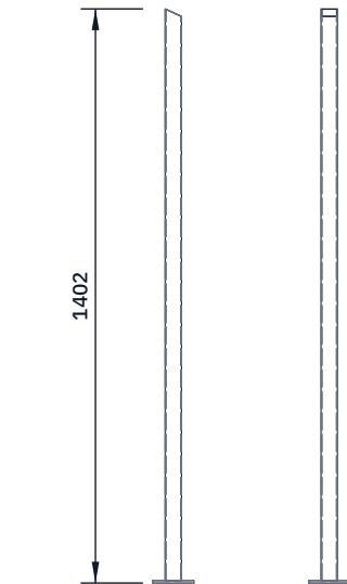
FRONT VIEW Scale 1:20; looking at the front (along +Y)
