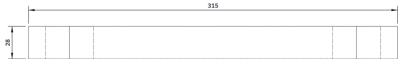
TOP VIEW Scale 1:2; looking down (along -Z)
