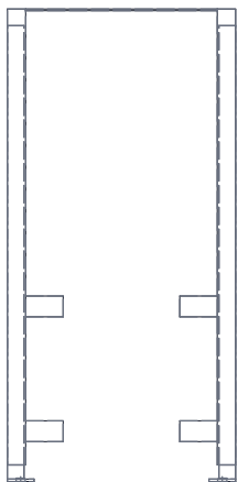
RIGHT VIEW Scale 1:10; looking at the right side (along -X)
