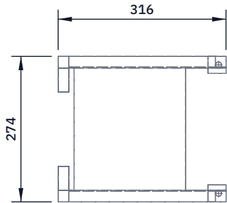
TOP VIEW Scale 1:10; looking down (along -Z)
