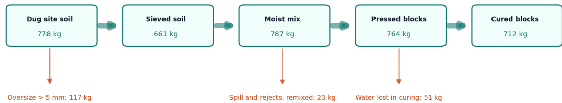
Figure 3. Material flow per 100 blocks, in kg (EPR-CAL-001 section 10). All values are estimates for a soil with 15 % oversize, 5 % cement and 10 % water.
