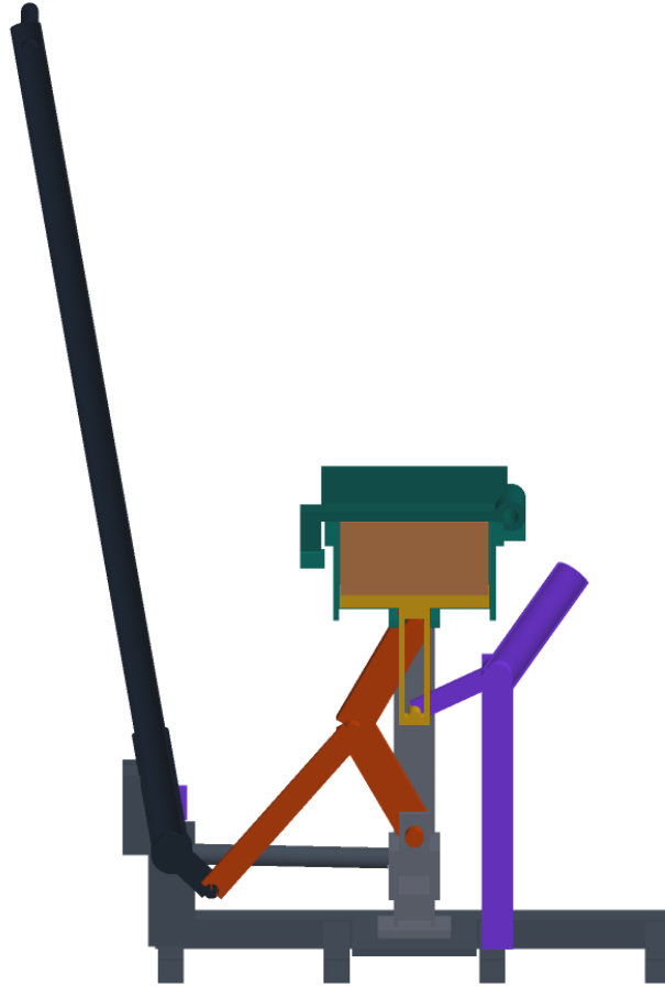
Figure 2. Section through the mold and linkage at the start of the stroke: loose soil (brown) above the piston and slotted push rod (yellow), toggle links (orange), lever hub, crank and connecting link on the left, eject seesaw (purple) on the right.
