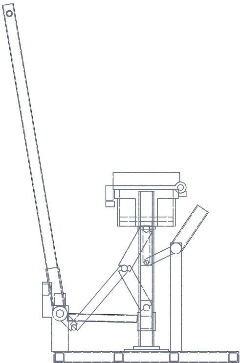
FRONT VIEW Scale 1:20
