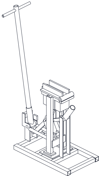
ISOMETRIC VIEW
