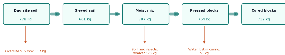
Figure 3. Material flow per 100 blocks, in kg (EPR-CAL-001 section 10). All values are estimates for a soil with 15 % oversize, 5 % cement and 10 % water.
