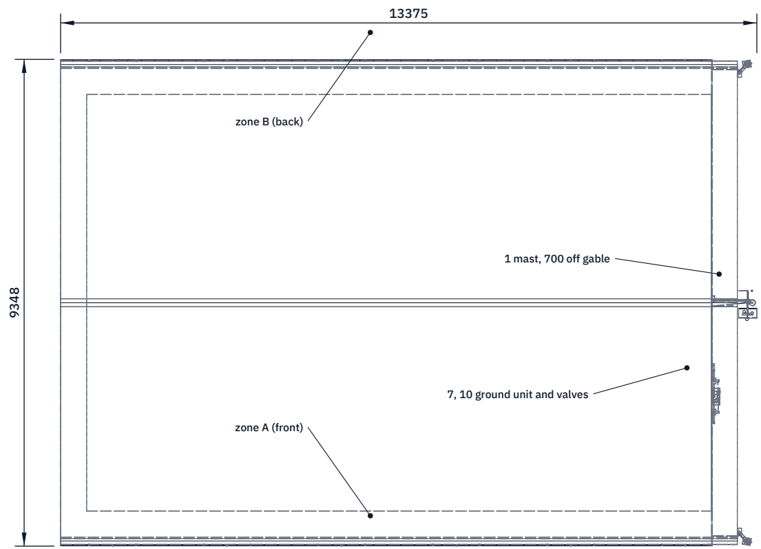
TOP VIEW
