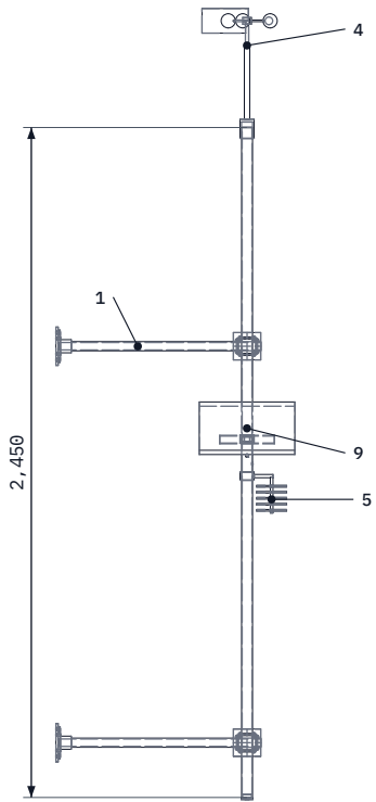
DETAIL A: MAST ASSEMBLY
