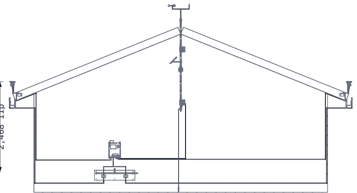
RIGHT VIEW
