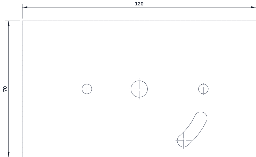
TOP VIEW Scale 1:1; looking down (along -Z)
