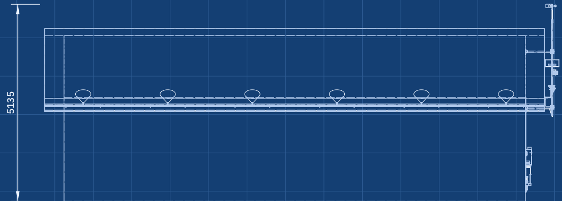
FRONT VIEW
