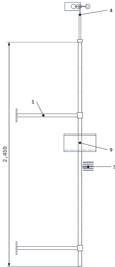
DETAIL A: MAST ASSEMBLY
