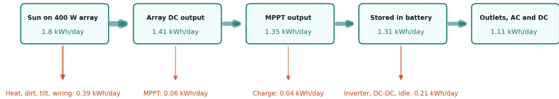
Figure 2. Daily energy flow at 4.5 kWh/m 2 /day global horizontal irradiation. All values are estimates from FCL-CAL-001.
