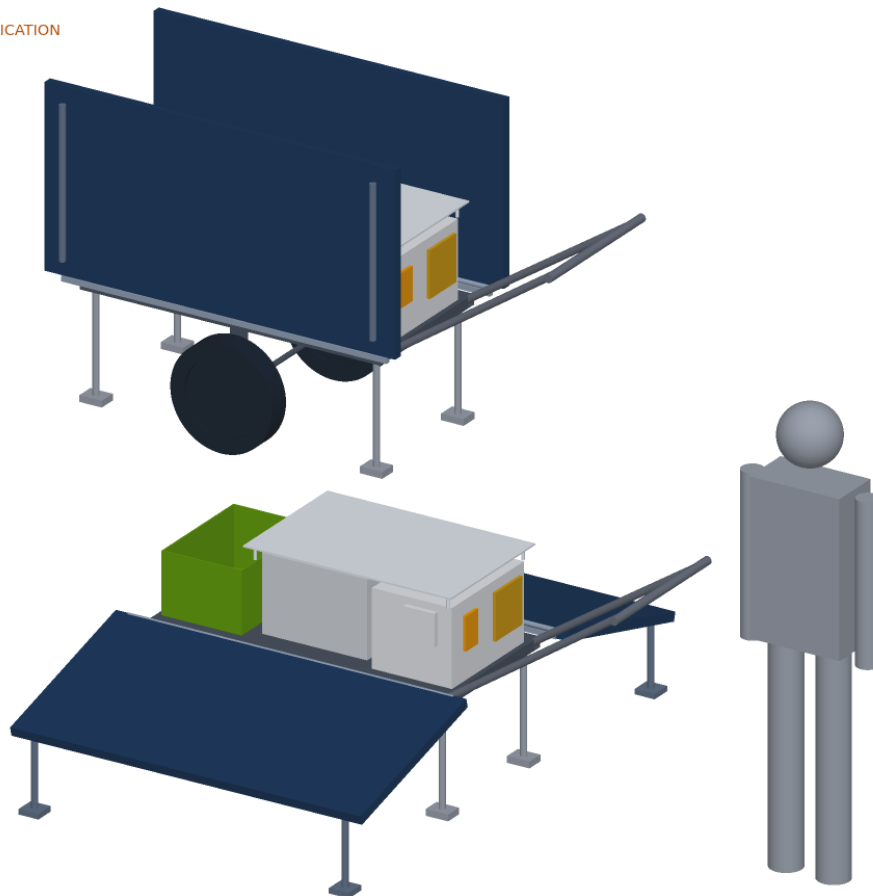
Figure 1. FieldCell deployed (front) and stowed for travel (behind), with a 1.75 m person for scale. Generated from the parametric model cad/src/model.py .
