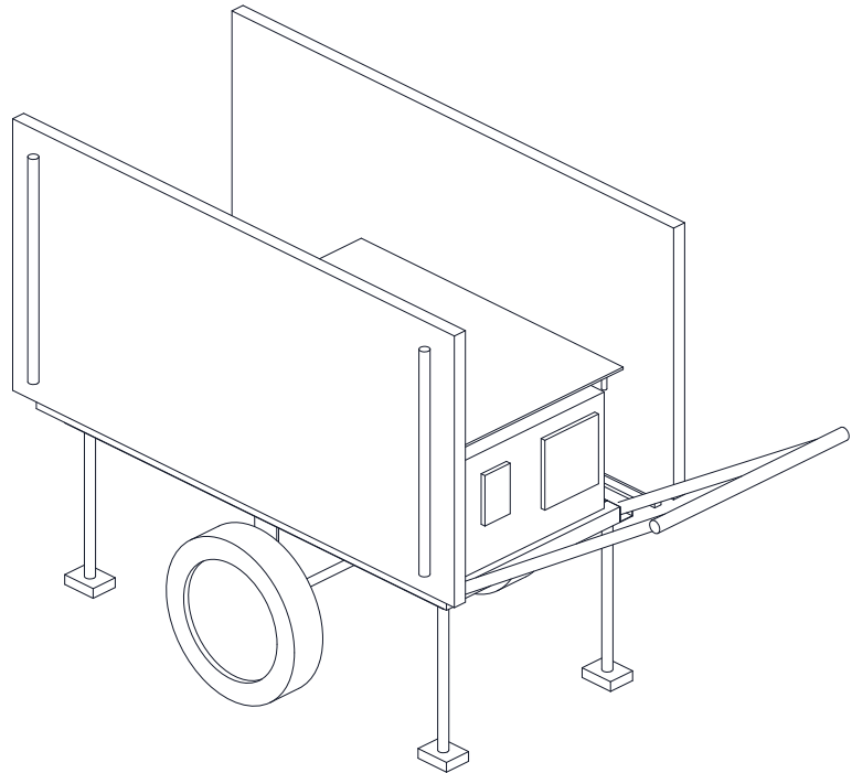
ISOMETRIC VIEW, STOWED FOR TRAVEL
