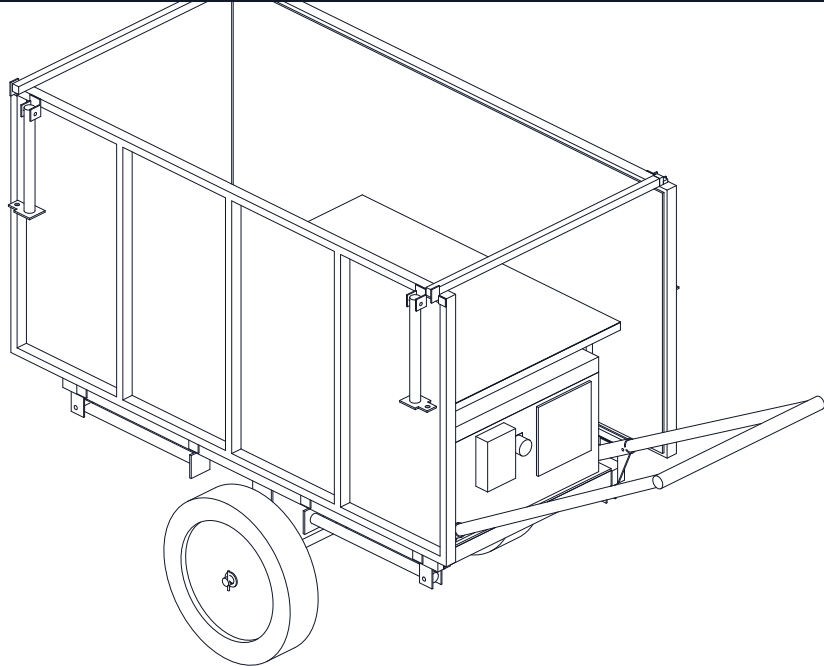
ISOMETRIC VIEW, STOWED FOR TRAVEL
