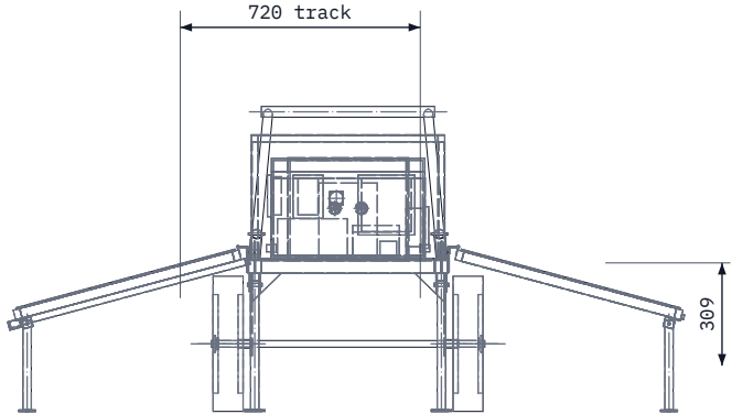
RIGHT VIEW
