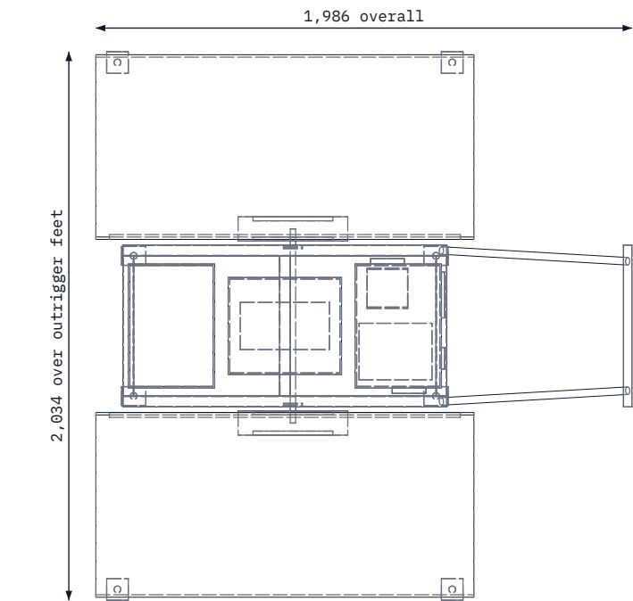
TOP VIEW Scale 1:25
