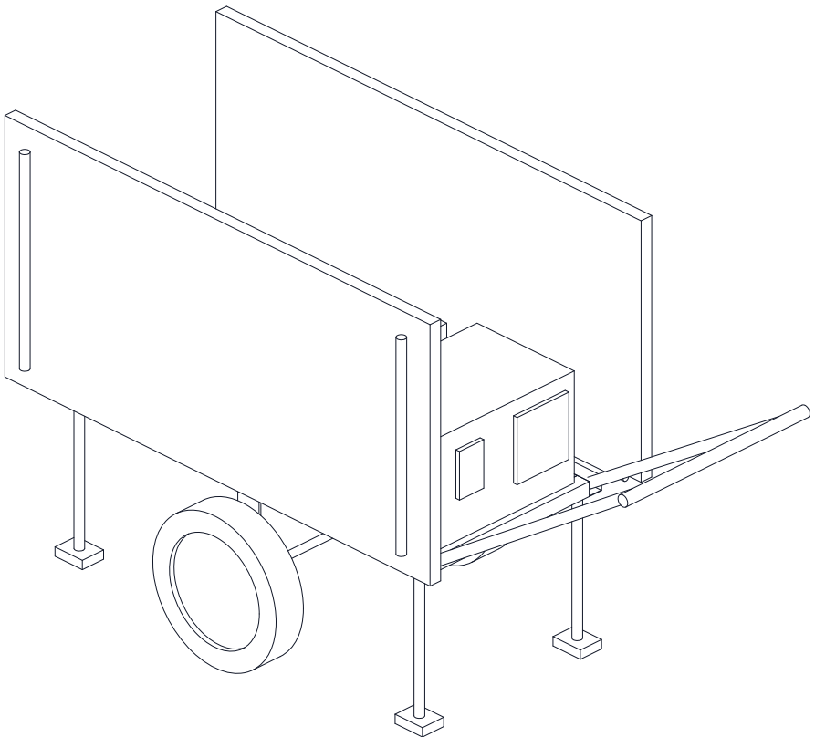
ISOMETRIC VIEW, STOWED FOR TRAVEL Not to scale
