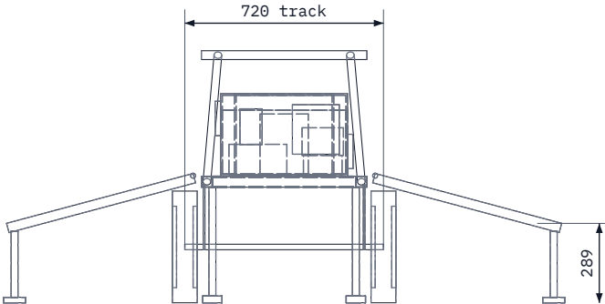
RIGHT VIEW Scale 1:25
