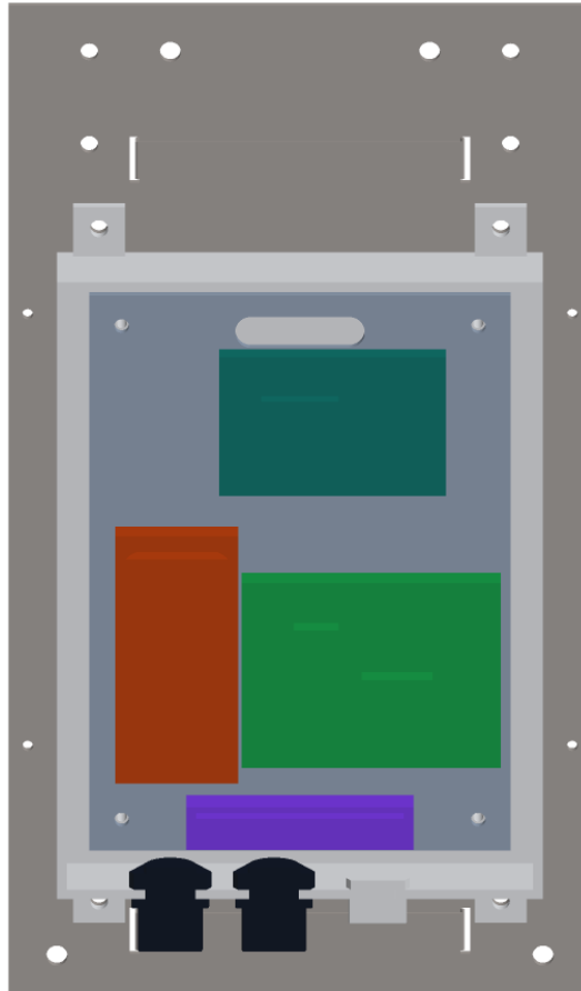
Figure 3. Cutaway from the front: cell (orange), power board (green) and controller (teal) on the internal plate.
