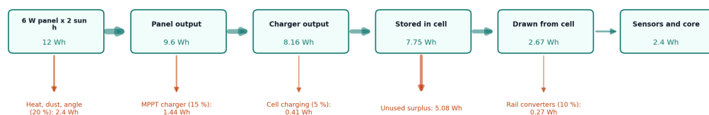
Figure 4. Daily energy flow in the worst month at the 100 mW design allowance (FND-CAL-001).
